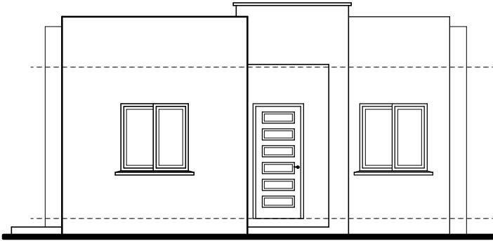
NORTH ELEVATION SCALE = 1/8" TO 1'-0"
