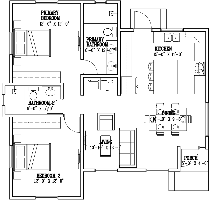
GROUND FLOOR PLAN SCALE = 1/8" TO 1'-0" 1050 SQ.FT
