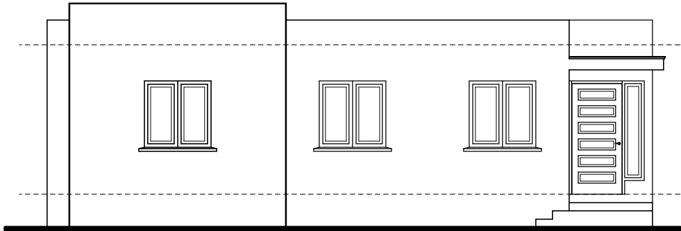
FRONT ELEVATION SCALE = 1/8" TO 1'-0"
