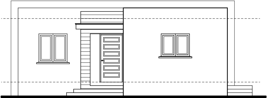
SIDE ELEVATION SCALE = 1/8" TO 1'-0"
