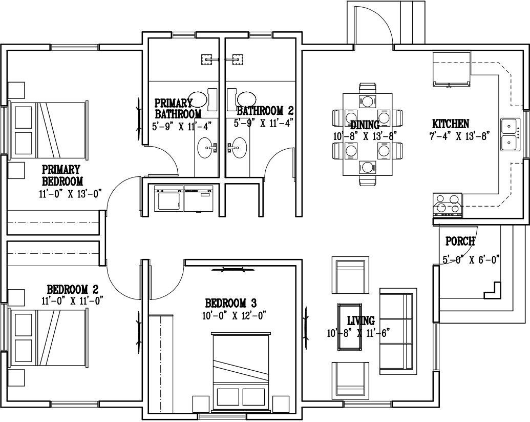
GROUND FLOOR PLAN SCALE = 1/8" TO 1'-0" 1216 SQ.FT
