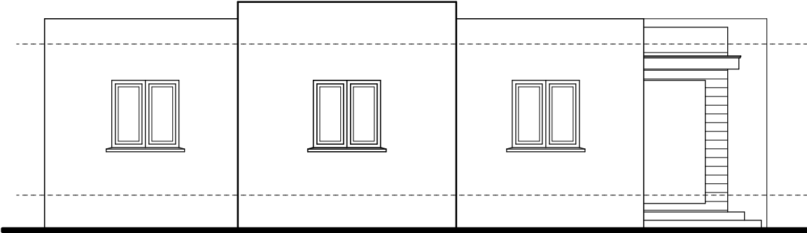
FRONT ELEVATION SCALE = 1/8" TO 1'-0"
